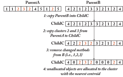
Figure 6: Example of crossover operator for clustering problems [11].
