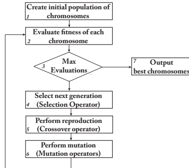
Figure 4: Different steps of a genetic algorithm.
