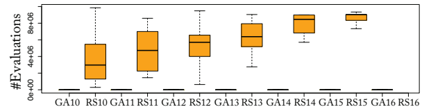
Figure 7: Box plots showing the number of fitness evaluations (#Evaluations) required by GA and RS. GAX and RSX label the box plots for the OrderItem with X methods.
